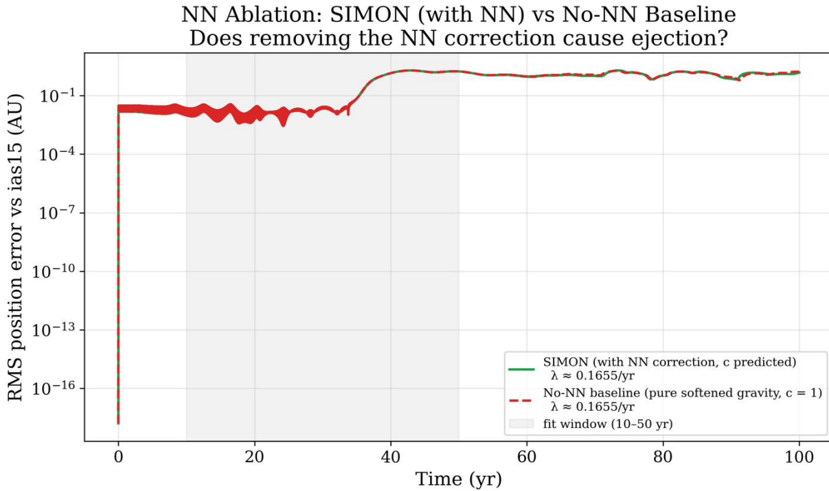
Figure 1. RMS position error vs ias15 over 100 years for SIMON (green) and No-NN baseline (red dashed). Both models track identically throughout — \lambda = 0.1655/\text{yr} for both, both bodies bounded. The curves are visually indistinguishable during the bounded phase. Final RMS differs by 0.13 AU (8.5%).
